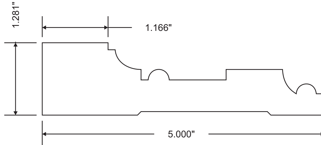
REVISED PROFILE
